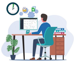
With DataDora
